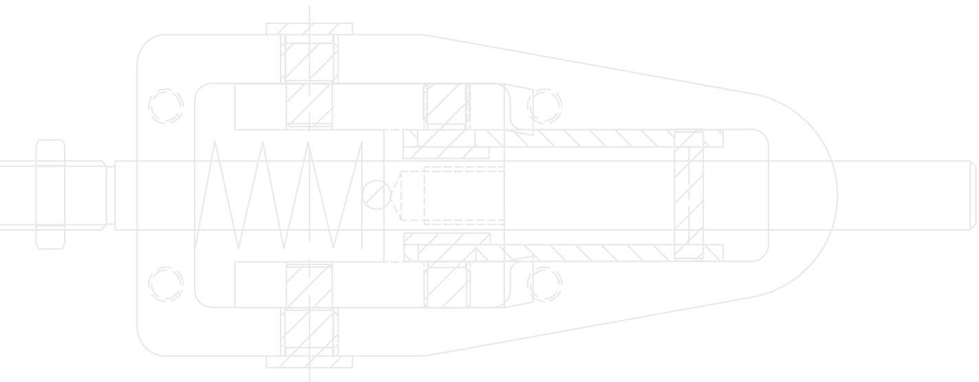
Protected gasket and hooks
